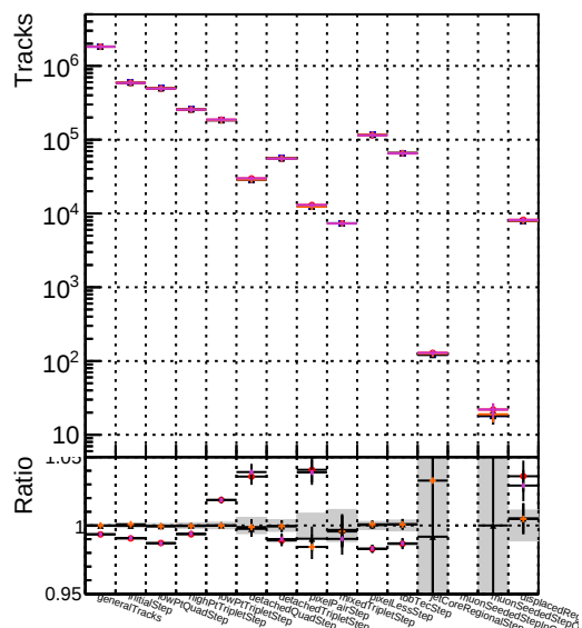
Number of tracks vs collection Legend: DOM original_step2_ttbbar-phase1-newgeom DOM mkFit_step2_ttbbar-phase1-newgeom DOM angle_step2_ttbbar-phase1-newgeom DOM fast_step2_ttbbar-phase1-newgeom DOM pixelCPEtemplate_step2_ttbbar-phase1-newgeom
