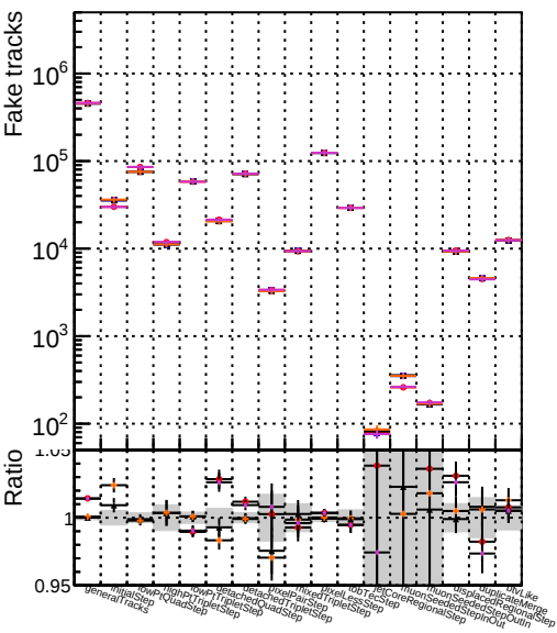
DOM original_step2_tbar-phase1-newgeom DOM mkFit_step2_tbar-phase1-newgeom DOM file_step2_tbar-phase1-newgeom DOM fastCPE_template_tbar-phase1-newgeom DOM pixelCPE1_template_step2_tbar-phase1-newgeom
