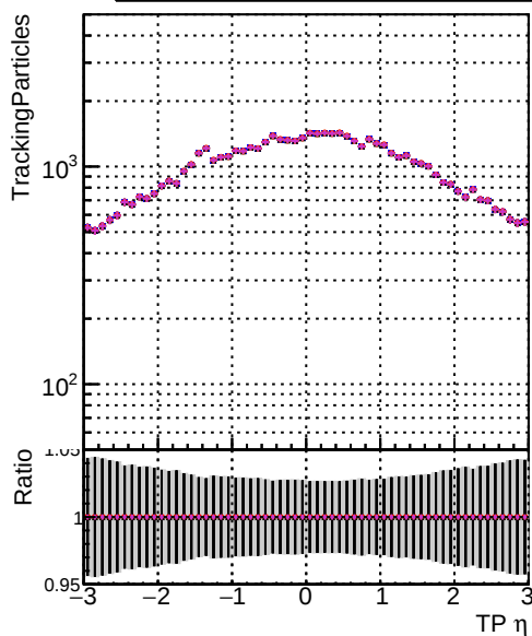
—•— DQM original_step2_ttbar-phase1-newgeom —•— DQM mkFit_step2_ttbar-phase1-newgeom —•— DQM angle_step2_ttbar-phase1-newgeom —•— DQM fast_step2_ttbar-phase1-newgeom —•— DQM pixelCPEtemplate_step2_ttbar-phase1-newgeom
