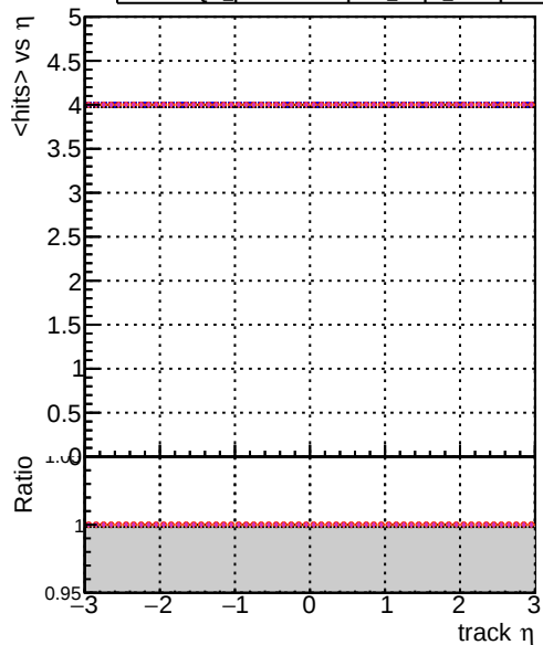
mean hit DOM original_step2_ttbbar-phase1-newgeom DOM mkrfit_step2_ttbbar-phase1-newgeom DOM angle_step2_ttbbar-phase1-newgeom DOM fast_step2_ttbbar-phase1-newgeom DOM pixelCPEtemplate_step2_ttbbar-phase1-newgeom
