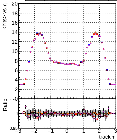
DOM original_step2_ttbbar-phase1-newgeom DOM mkrfit_step2_ttbbar-phase1-newgeom DOM angle_step2_ttbbar-phase1-newgeom DOM fast_step2_ttbbar-phase1-newgeom DOM pixelCPEtemplate_step2_ttbbar-phase1-newgeom mean hit
