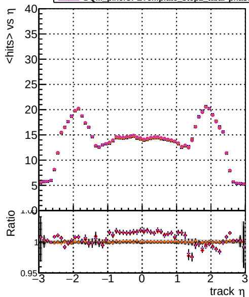
mean hits vs \eta Legend: DOM original_step2_ttbbar-phase1-newgeom DOM mkrfit_step2_ttbbar-phase1-newgeom DOM angle_step2_ttbbar-phase1-newgeom DOM fast_step2_ttbbar-phase1-newgeom DOM pixelCPEtemplate_step2_ttbbar-phase1-newgeom
