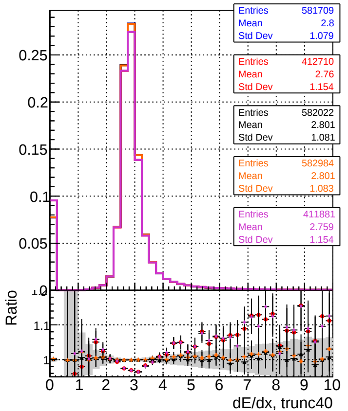
— DQM_original_step2_ttbar-phase1-newgeom — DQM_mkFit_step2_ttbar-phase1-newgeom — DQM_angle_step2_ttbar-phase1-newgeom — DQM_fast_step2_ttbar-phase1-newgeom — DQM_pixelCPETemplate_step2_ttbar-phase1-newgeom
