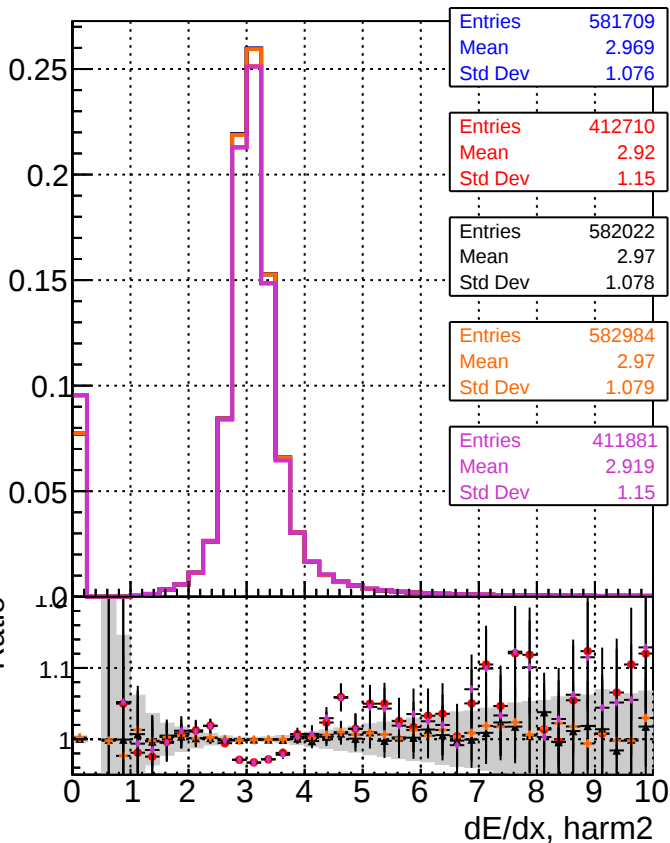
— DQM_original_step2_ttbar-phase1-newgeom — DQM_mkFit_step2_ttbar-phase1-newgeom — DQM_angle_step2_ttbar-phase1-newgeom — DQM_fast_step2_ttbar-phase1-newgeom — DQM_pixelCPETemplate_step2_ttbar-phase1-newgeom
