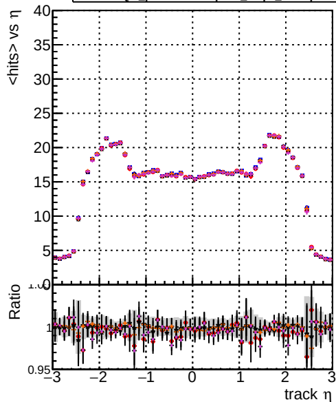
DOM original_step2_ttbbar-phase1-newgeom DOM mkFit_step2_ttbbar-phase1-newgeom DOM angle_step2_ttbbar-phase1-newgeom DOM fast_step2_ttbbar-phase1-newgeom DOM pixelCPEtemplate_step2_ttbbar-phase1-newgeom mean hits
