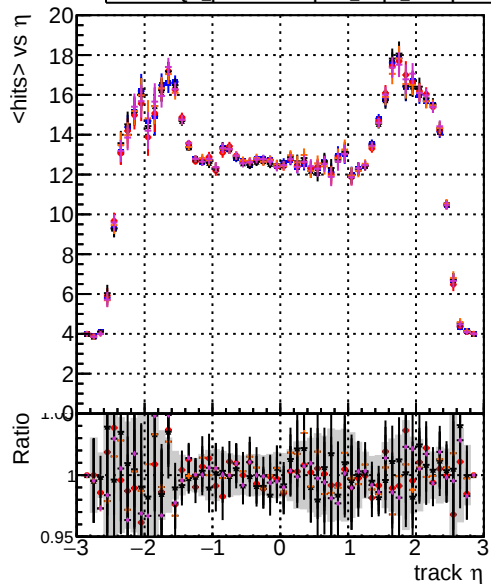
mean hit DOM original_step2_ttbare-phase1-newgeom DOM mkFit_step2_ttbare-phase1-newgeom DOM angle_step2_ttbare-phase1-newgeom DOM fast_step2_ttbare-phase1-newgeom DOM pixelCPEtemplate_step2_ttbare-phase1-newgeom
