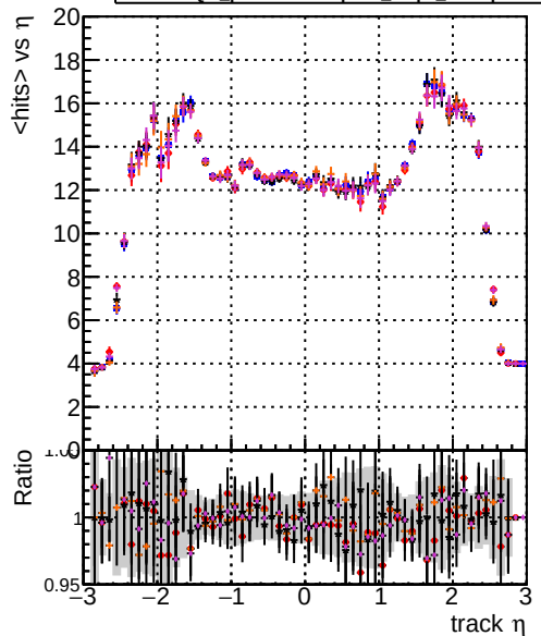
DOM original_step2_ttbare-phase1-newgeom DOM mkFit_step2_ttbare-phase1-newgeom DOM angle_step2_ttbare-phase1-newgeom DOM fast_step2_ttbare-phase1-newgeom DOM pixelCPEtemplate_step2_ttbare-phase1-newgeom
