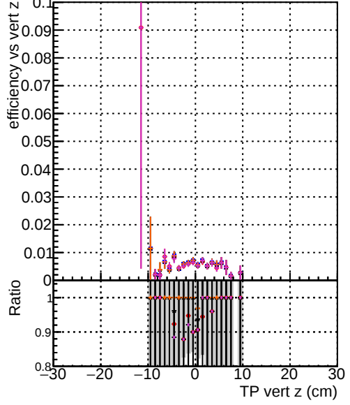
Efficiency vs. sim PV z — DOM original_step2_ttbar-phase1-newgeom — DOM mkr_fit_step2_ttbar-phase1-newgeom — DOM angle_step2_ttbar-phase1-newgeom — DOM fast_step2_ttbar-phase1-newgeom — DOM pixelCPEtemplate_step2_ttbar-phase1-newgeom
