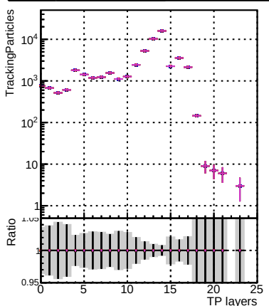
N of sim — DQM_fast_step2_ttbar-phase1-newgeom — DQM_pixelCPETemplate_step2_ttbar-phase1-newgeom
