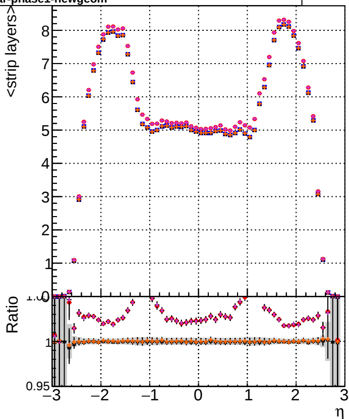
Legend for STRIP hits plots: DQM_original_step2_ttbar-phase1-newgeom (blue squares) DQM_mkFit_step2_ttbar-phase1-newgeom (red circles) DQM_angle_step2_ttbar-phase1-newgeom (black triangles) DQM_fast_step2_ttbar-phase1-newgeom (orange diamonds) DQM_pixelCPETemplate_step2_ttbar-phase1-newgeom (magenta squares)
