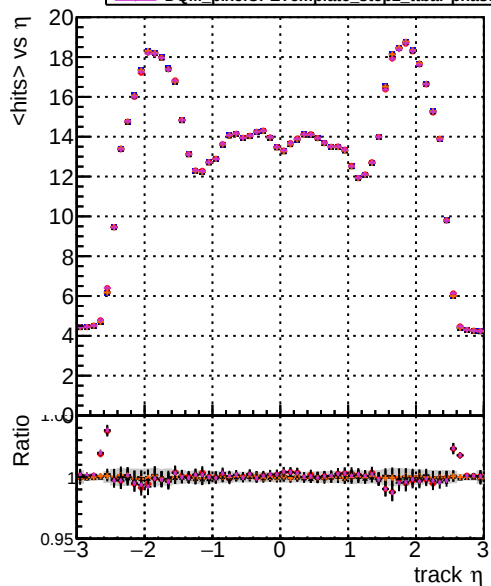
mean hits DOM original_step2_ttbbar-phase1-newgeom DOM mkrfit_step2_ttbbar-phase1-newgeom DOM angle_step2_ttbbar-phase1-newgeom DOM fast_step2_ttbbar-phase1-newgeom DOM pixelCPEtemplate_step2_ttbbar-phase1-newgeom
