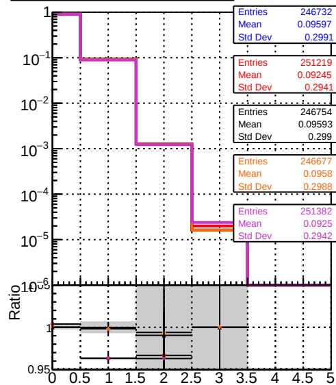
mean hits DOM original_step2_ttbbar-phase1-newgeom DOM mkrfit_step2_ttbbar-phase1-newgeom DOM angle_step2_ttbbar-phase1-newgeom DOM fast_step2_ttbbar-phase1-newgeom DOM pixelCPEtemplate_step2_ttbbar-phase1-newgeom
