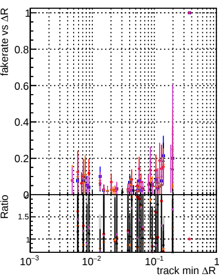
Fake rate vs \Delta R(\text{track, jet}) Legend: DOM (blue) original_step2 (red) tthar_phase1-newgeom (green) angle_step2 (orange) tthar_phase1-newgeom (purple) fixedCP-Template_step2 (brown)
