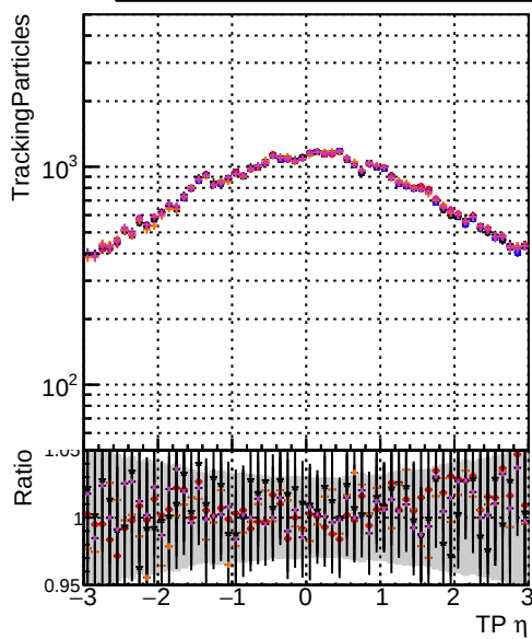
— DOM_original_step2_ttbar-phase1-newgeom — DOM_mkFit_step2_ttbar-phase1-newgeom — DOM_angle_step2_ttbar-phase1-newgeom — DOM_fast_step2_ttbar-phase1-newgeom — DOM_pixelCPEtemplate_step2_ttbar-phase1-newgeom
