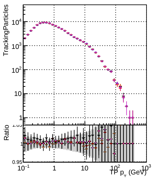
— DOM_original_step2_ttbar-phase1-newgeom — DOM_mkFit_step2_ttbar-phase1-newgeom — DOM_angle_step2_ttbar-phase1-newgeom — DOM_fast_step2_ttbar-phase1-newgeom — DOM_pixelCPEtemplate_step2_ttbar-phase1-newgeom
