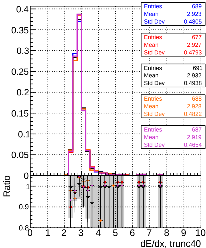
— DQM original_step2_ttbar-phase1-newgeom — DQM mkFit_step2_ttbar-phase1-newgeom — DQM angle_step2_ttbar-phase1-newgeom — DQM fast_step2_ttbar-phase1-newgeom — DQM pixelCPETemplate_step2_ttbar-phase1-newgeom
