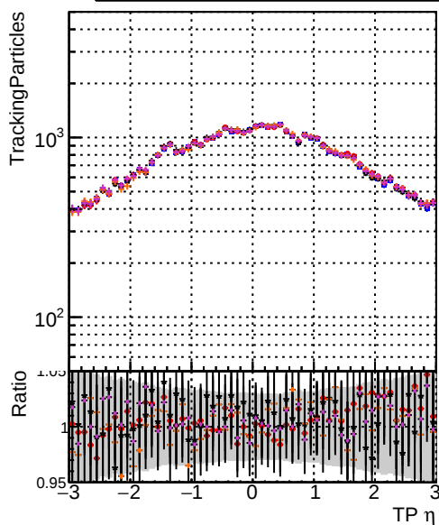
— DQM_original_step2_ttbar-phase1-newgeom — mkFit_step2_ttbar-phase1-newgeom — DQM_angle_step2_ttbar-phase1-newgeom — DQM_fast_step2_ttbar-phase1-newgeom — DQM_pixelCPEtemplate_step2_ttbar-phase1-newgeom
