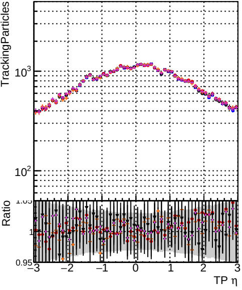
— DOM original_step2_ttbar-phase1-newgeom — DOM mkFit_step2_ttbar-phase1-newgeom — DOM angle_step2_ttbar-phase1-newgeom — DOM fast_step2_ttbar-phase1-newgeom — DOM pixelCPEtemplate_step2_ttbar-phase1-newgeom
