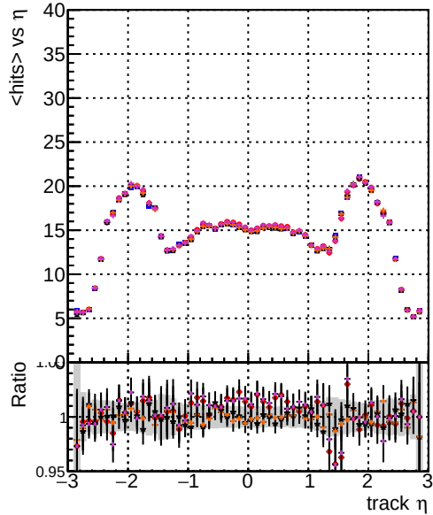
DOM original_step2_ttbart-phase1-newgeom DOM mkFit_step2_ttbart-phase1-newgeom DOM angle_step2_ttbart-phase1-newgeom DOM fast_step2_ttbart-phase1-newgeom DOM pixelCPEtemplate_step2_ttbart-phase1-newgeom mean hits
