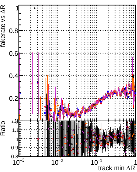
Fake rate vs \Delta R(\text{track, jet}) Legend: DOM (blue) original_step2 (orange) tthar-phase1-newgeom (green) angle_step2 (red) tthar-phase1-newgeom (purple) fixedCP-Template-step2 (magenta)
