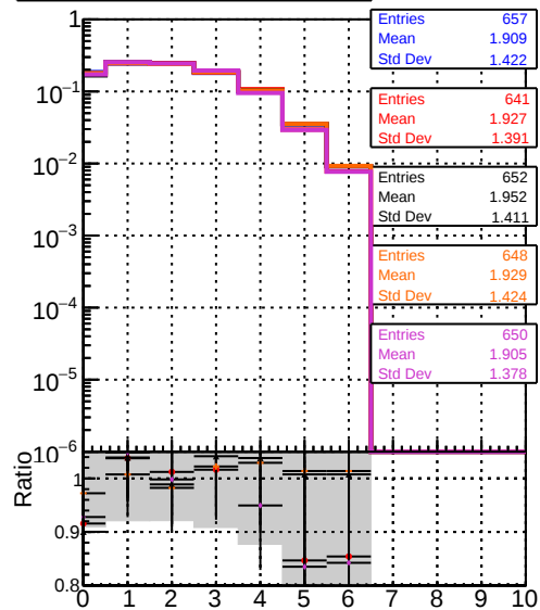
DOM original_step2_ttbare-phase1-newgeom DOM mkFit_step2_ttbare-phase1-newgeom DOM angle_step2_ttbare-phase1-newgeom DOM fast_step2_ttbare-phase1-newgeom DOM pixelCPEtemplate_step2_ttbare-phase1-newgeom
