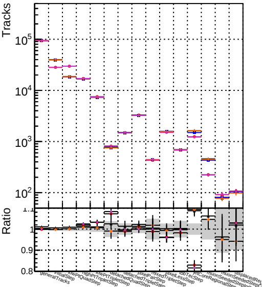
Number Legend Model 1 DDM original_step2_ttb-ar-phase1-newgeom 2 DDM mkf-it_step2_ttb-ar-phase1-newgeom 3 DDM angle_step2_ttb-ar-phase1-newgeom 4 DDM fast_step2_ttb-ar-phase1-newgeom 5 DDM pixelCPEtemplate_step2_ttb-ar-phase1-newgeom
