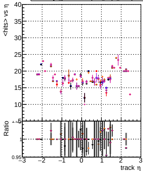
DOM original_step2_ttbar-phase1-newgeom DOM mkFit_step2_ttbar-phase1-newgeom DOM angle_step2_ttbar-phase1-newgeom DOM fast_step2_ttbar-phase1-newgeom DOM pixelCPEtemplate_step2_ttbar-phase1-newgeom
