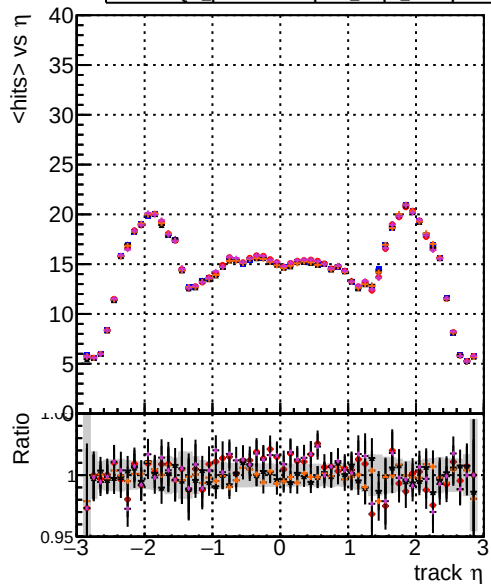
DOM original step2 ttbar-phase1-newgeom DOM mkFit step2 ttbar-phase1-newgeom DOM angle step2 ttbar-phase1-newgeom DOM fast step2 ttbar-phase1-newgeom DOM pixelCPE template step2 ttbar-phase1-newgeom mean hit
