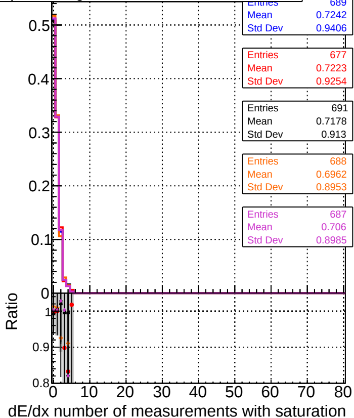
DQM_original_step2_ttbar-phase1-newgeom DQM_mkFit_step2_ttbar-phase1-newgeom DQM_angle_step2_ttbar-phase1-newgeom DQM_fast_step2_ttbar-phase1-newgeom DQM_pixelCPETemplate_step2_ttbar-phase1-newgeom
