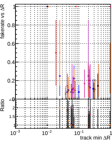
Fake rate vs \Delta R(\text{track}, \text{jet}) Legend: DOM (blue) original (red) step2 (orange) tth (purple) phase1 (green) newgeom (black)
