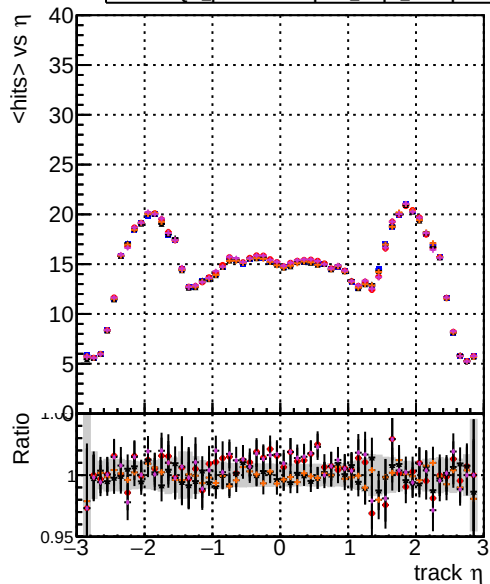
DOM original_step2_ttbbar-phase1-newgeom mkFit_step2_ttbbar-phase1-newgeom DOM angle_step2_ttbbar-phase1-newgeom DOM fast_step2_ttbbar-phase1-newgeom DOM pixelCPEtemplate_step2_ttbbar-phase1-newgeom mean hit
