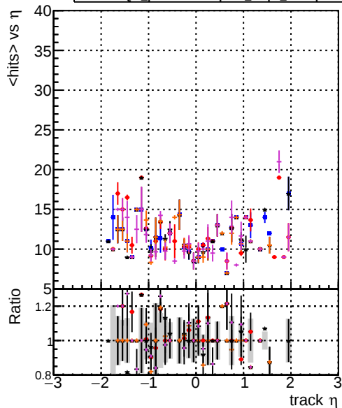
mean hit DQM original_step2_ttbar-phase1-newgeom mkFit_step2_ttbar-phase1-newgeom DQM angle_step2_ttbar-phase1-newgeom DQM fast_step2_ttbar-phase1-newgeom DQM pixelCPEtemplate_step2_ttbar-phase1-newgeom
