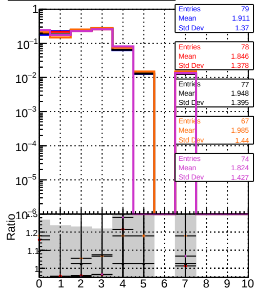
mean hit DQM original_step2_ttbar-phase1-newgeom mkFit_step2_ttbar-phase1-newgeom DQM angle_step2_ttbar-phase1-newgeom DQM fast_step2_ttbar-phase1-newgeom DQM pixelCPEtemplate_step2_ttbar-phase1-newgeom
