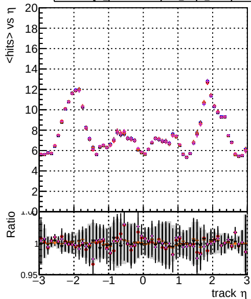
mean hit DOM original_step2_ttbbar-phase1-newgeom DOM mkFit_step2_ttbbar-phase1-newgeom DOM angle_step2_ttbbar-phase1-newgeom DOM fast_step2_ttbbar-phase1-newgeom DOM pixelCPEtemplate_step2_ttbbar-phase1-newgeom
