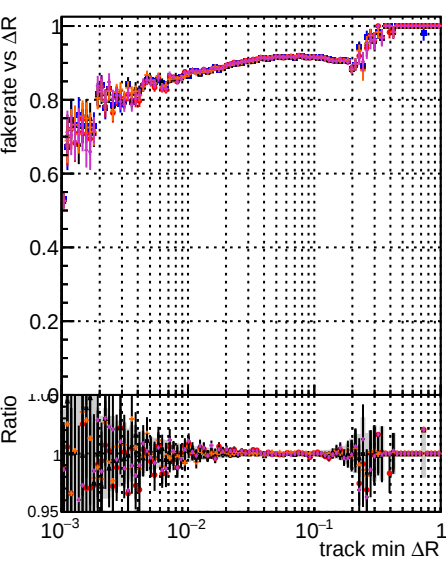
Fake rate vs \Delta R(\text{track, jet}) DOM original step2 tth phase1 newgeom original step2 tth phase1 newgeom fixerCPE template step2 tth phase1 newgeom
