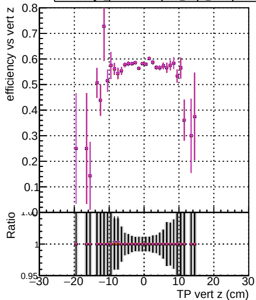
Efficiency vs. sim PV z — DOM original_step2_ttb̄r-phase1-newgeom — DOM mkrfit_step2_ttb̄r-phase1-newgeom — DOM angle_step2_ttb̄r-phase1-newgeom — DOM fast_step2_ttb̄r-phase1-newgeom — DOM pixelCPEtemplate_step2_ttb̄r-phase1-newgeom
