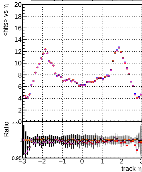
mean hits DOM original_step2_ttbbar-phase1-newgeom DOM mkFit_step2_ttbbar-phase1-newgeom DOM angle_step2_ttbbar-phase1-newgeom DOM fast_step2_ttbbar-phase1-newgeom DOM pixelCPEtemplate_step2_ttbbar-phase1-newgeom
