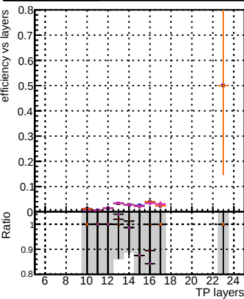
Efficiency vs hit DOM_original_step2_ttbar-phase1-newgeom DOM_mkFit_step2_ttbar-phase1-newgeom DOM_angle_step2_ttbar-phase1-newgeom DOM_fast_step2_ttbar-phase1-newgeom DOM_pixelCPETemplate_step2_ttbar-phase1-newgeom
