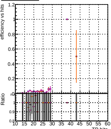
Efficiency vs hit DOM_original_step2_ttbar-phase1-newgeom DOM_mkFit_step2_ttbar-phase1-newgeom DOM_angle_step2_ttbar-phase1-newgeom DOM_fast_step2_ttbar-phase1-newgeom DOM_pixelCPETemplate_step2_ttbar-phase1-newgeom
