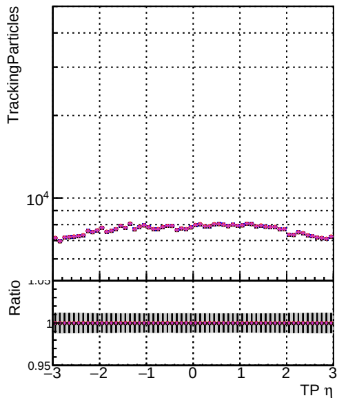
—•— DQM_original_step2_ttbar-phase1-newgeom —•— DQM_mkfit_step2_ttbar-phase1-newgeom —•— DQM_angle_step2_ttbar-phase1-newgeom —•— DQM_fast_step2_ttbar-phase1-newgeom —•— DQM_pixelCPEtemplate_step2_ttbar-phase1-newgeom
