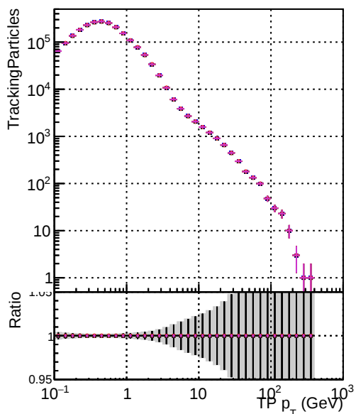
—•— DQM_original_step2_ttbar-phase1-newgeom —•— DQM_mkfit_step2_ttbar-phase1-newgeom —•— DQM_angle_step2_ttbar-phase1-newgeom —•— DQM_fast_step2_ttbar-phase1-newgeom —•— DQM_pixelCPEtemplate_step2_ttbar-phase1-newgeom
