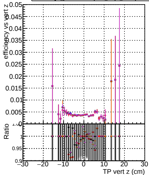
Efficiency vs vert z — DOM original_step2_ttbbar-phase1-newgeom — DOM mkrfit_step2_ttbbar-phase1-newgeom — DOM angle_step2_ttbbar-phase1-newgeom — DOM fast_step2_ttbbar-phase1-newgeom — DOM pixelCPEtemplate_step2_ttbbar-phase1-newgeom
