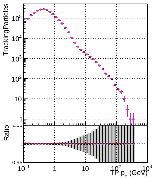
—•— DOM_original_step2_ttbar-phase1-newgeom —•— DOM_mkFit_step2_ttbar-phase1-newgeom —•— DOM_angle_step2_ttbar-phase1-newgeom —•— DOM_fast_step2_ttbar-phase1-newgeom —•— DOM_pixelCPEtemplate_step2_ttbar-phase1-newgeom
