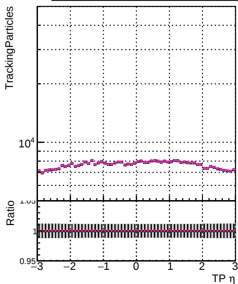
—•— DOM_original_step2_ttbar-phase1-newgeom —•— DOM_mkFit_step2_ttbar-phase1-newgeom —•— DOM_angle_step2_ttbar-phase1-newgeom —•— DOM_fast_step2_ttbar-phase1-newgeom —•— DOM_pixelCPEtemplate_step2_ttbar-phase1-newgeom
