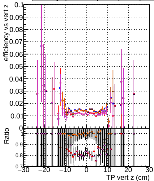
Efficiency vs vert z — DOM original_step2_ttbar-phase1-newgeom — DOM mkrfit_step2_ttbar-phase1-newgeom — DOM angle_step2_ttbar-phase1-newgeom — DOM fast_step2_ttbar-phase1-newgeom — DOM pixelCPEtemplate_step2_ttbar-phase1-newgeom
