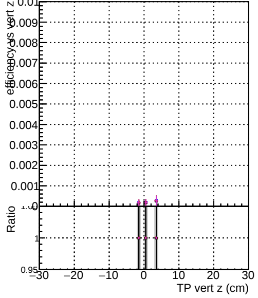
Efficiency vs vert z DOM original_step2_ttbar-phase1-newgeom DOM mkFit_step2_ttbar-phase1-newgeom DOM angle_step2_ttbar-phase1-newgeom DOM fast_step2_ttbar-phase1-newgeom DOM pixelCPE_template_step2_ttbar-phase1-newgeom
