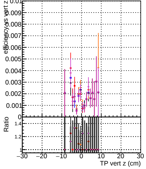
Efficiency vs vert z — DQM original_step2 ttbar-phase1-newgeom — DQM mkFit_step2 ttbar-phase1-newgeom — DQM angle_step2 ttbar-phase1-newgeom — DQM fast_step2 ttbar-phase1-newgeom — DQM pixelCPEtemplate_step2 ttbar-phase1-newgeom
