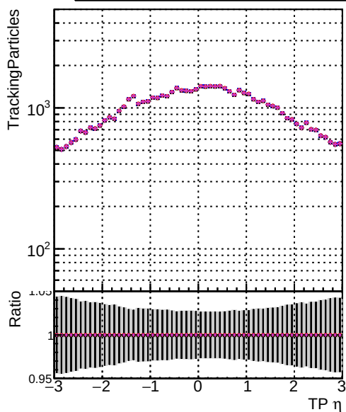
— DQM original_step2_ttbar-phase1-newgeom — DQM mkFit_step2_ttbar-phase1-newgeom — DQM angle_step2_ttbar-phase1-newgeom — DQM fast_step2_ttbar-phase1-newgeom — DQM pixelCPEtemplate_step2_ttbar-phase1-newgeom
