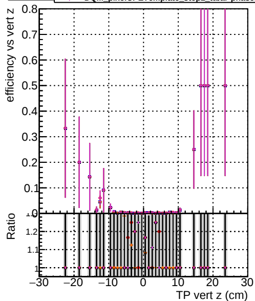
Efficiency vs vert z — DOM original_step2_ttbar-phase1-newgeom — mkFit_step2_ttbar-phase1-newgeom — DOM_angle_step2_ttbar-phase1-newgeom — DOM_fast_step2_ttbar-phase1-newgeom — DOM_pixelCPEtemplate_step2_ttbar-phase1-newgeom
