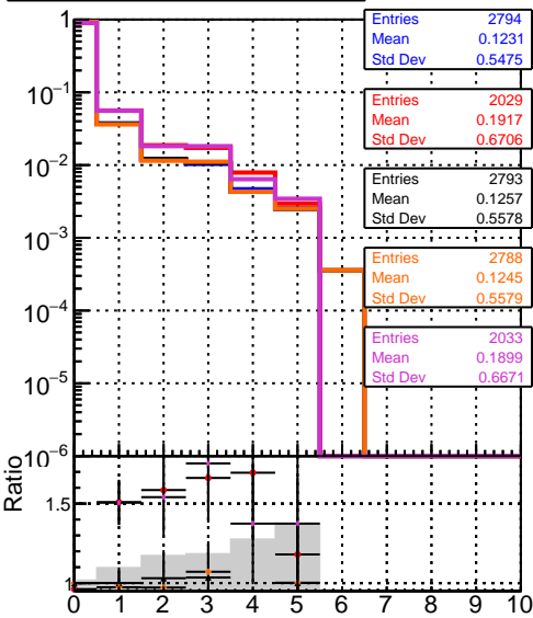
mean hit — DQM original_step2_ttbbar-phase1-newgeom — DQM mkrfit_step2_ttbbar-phase1-newgeom — DQM angle_step2_ttbbar-phase1-newgeom — DQM fast_step2_ttbbar-phase1-newgeom — DQM pixelCPEtemplate_step2_ttbbar-phase1-newgeom
