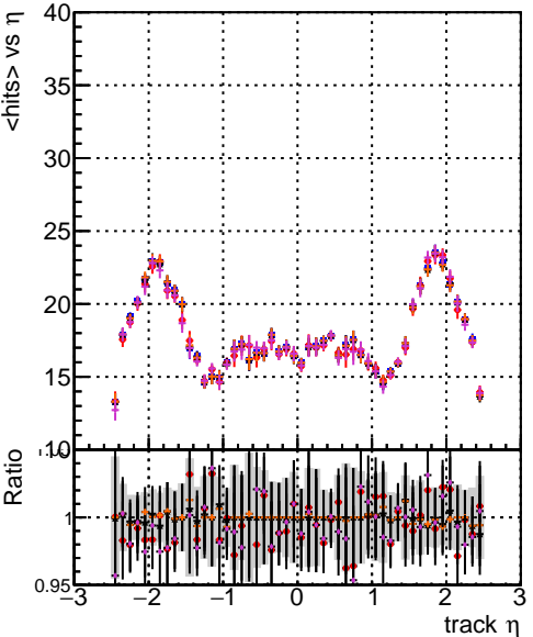
mean hit — DQM original_step2_ttbbar-phase1-newgeom — DQM mkrfit_step2_ttbbar-phase1-newgeom — DQM angle_step2_ttbbar-phase1-newgeom — DQM fast_step2_ttbbar-phase1-newgeom — DQM pixelCPEtemplate_step2_ttbbar-phase1-newgeom
