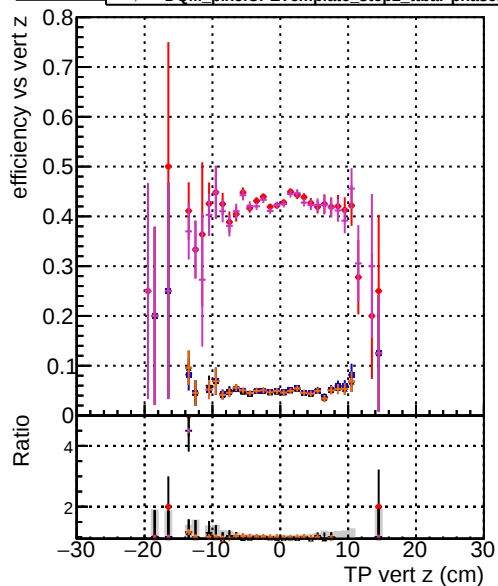
Efficiency vs vert z — DOM original_step2_ttbar-phase1-newgeom — DOM mkFit_step2_ttbar-phase1-newgeom — DOM angle_step2_ttbar-phase1-newgeom — DOM fast_step2_ttbar-phase1-newgeom — DOM pixelCPEtemplate_step2_ttbar-phase1-newgeom
