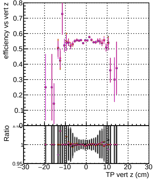
Efficiency vs vert z — DOM original_step2_ttbarm-phase1-newgeom — DOM mkFit_step2_ttbarm-phase1-newgeom — DOM angle_step2_ttbarm-phase1-newgeom — DOM fast_step2_ttbarm-phase1-newgeom — DOM pixelCPEtemplate_step2_ttbarm-phase1-newgeom
