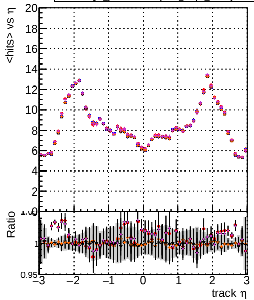
DOM-original_step2_ttbbar-phase1-newgeom DOM-mkFit_step2_ttbbar-phase1-newgeom DOM-angle_step2_ttbbar-phase1-newgeom DOM-fast_step2_ttbbar-phase1-newgeom DOM-pixelCPEtemplate_step2_ttbbar-phase1-newgeom mean hit
