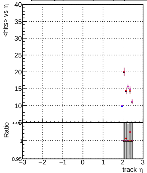
DOM original_step2_pt200_eta2p0to2p5 DOM mkFit_step2_pt200_eta2p0to2p5 DOM angle_step2_pt200_eta2p0to2p5 DOM fast_step2_pt200_eta2p0to2p5 DOM pixelCPEtemplate_step2_pt200_eta2p0to2p5
