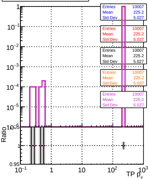
N of simulated tracks vs pT
