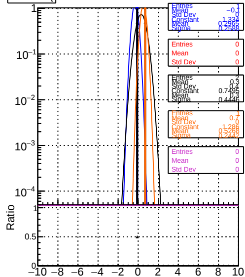
DOM original step2 - pt200 eta2p0to2p5 DOM original step2 - pt200 eta2p0to2p5 DOM original step2 - pt200 eta2p0to2p5 DOM original step2 - pt200 eta2p0to2p5
