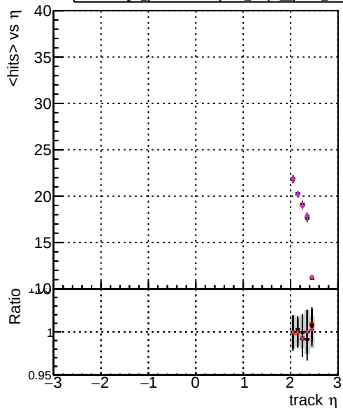
DOM original_step2_pt200_eta2p0to2p5 DOM mkrfit_step2_pt200_eta2p0to2p5 DOM angle_step2_pt200_eta2p0to2p5 DOM fast_step2_pt200_eta2p0to2p5 DOM pixelCPEtemplate_step2_pt200_eta2p0to2p5 mean hits
